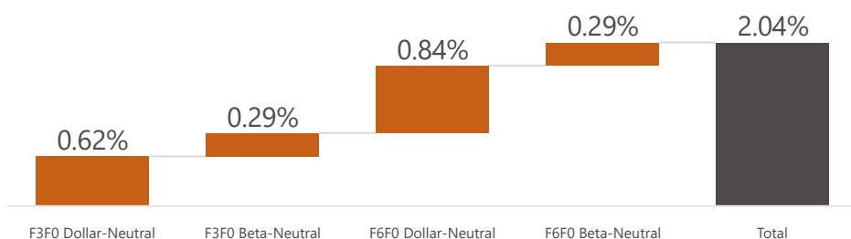
1y Backwardation Measure
