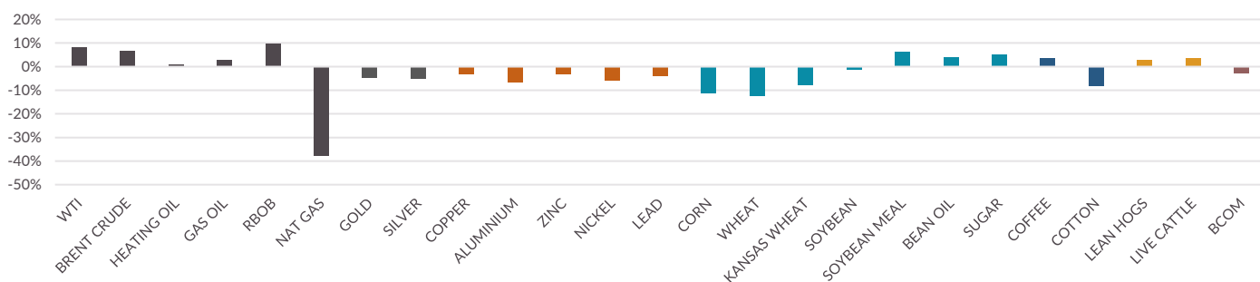
1y Backwardation Measure
